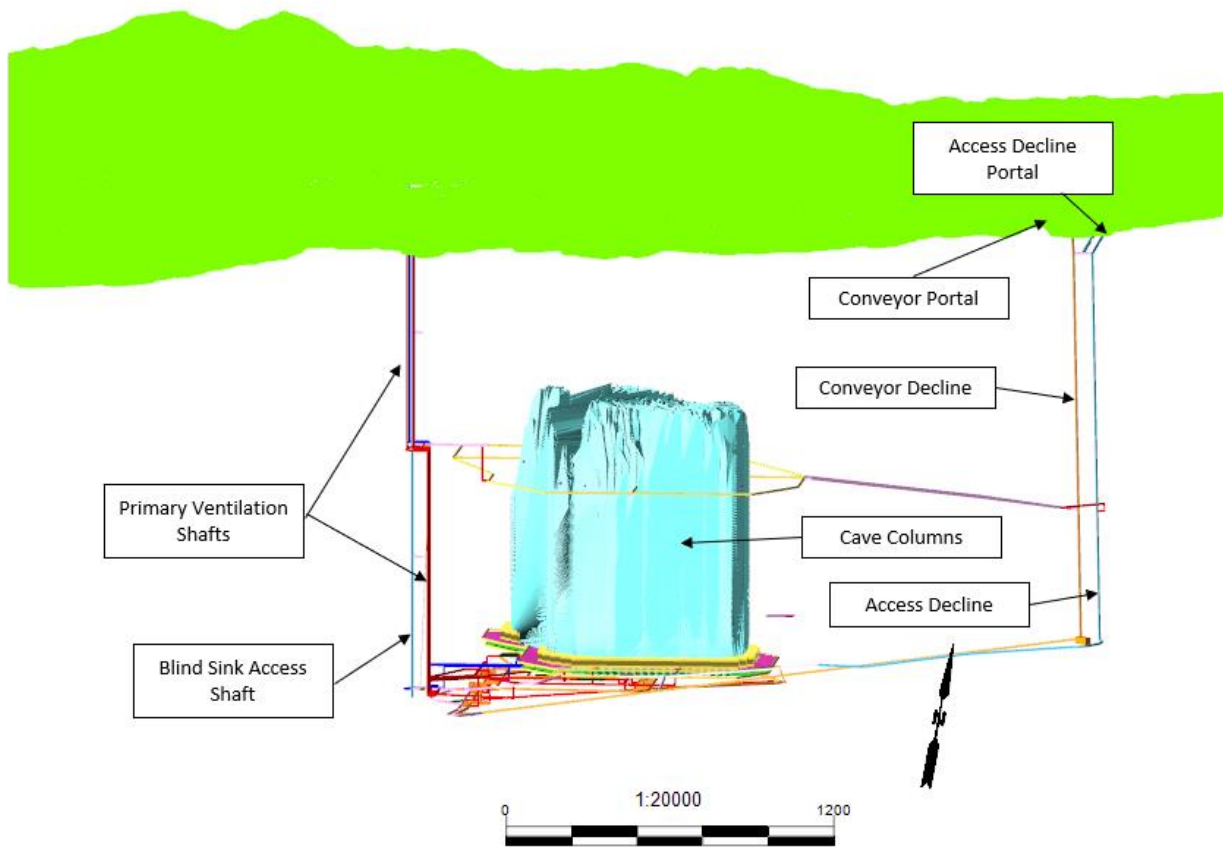
Figure 1: Isometric view of the lateral and vertical accesses in the Cascabel project Alpa underground mine
