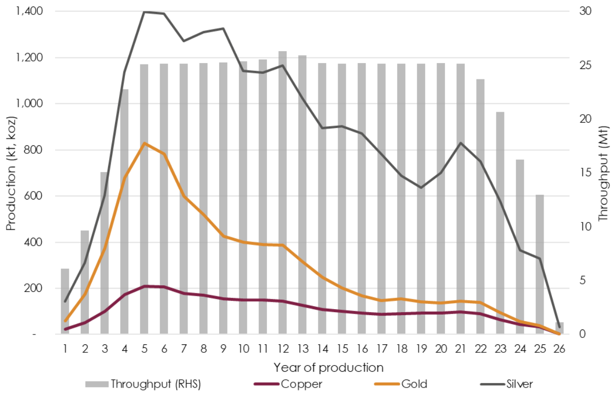
Figure 5: Production profile
