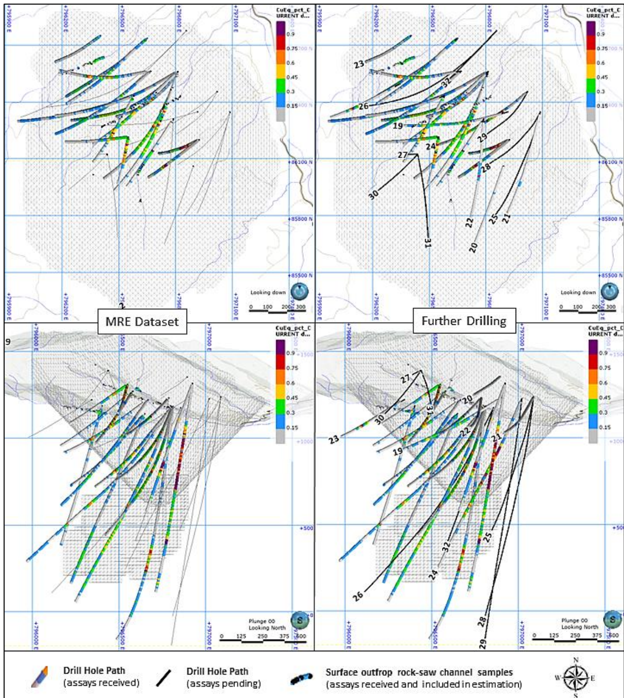
Figure 2: Comparative plan (TOP) and section (BOTTOM) views of TAM MRE dataset (LEFT) and the current additional drilling achieved (RIGHT).
