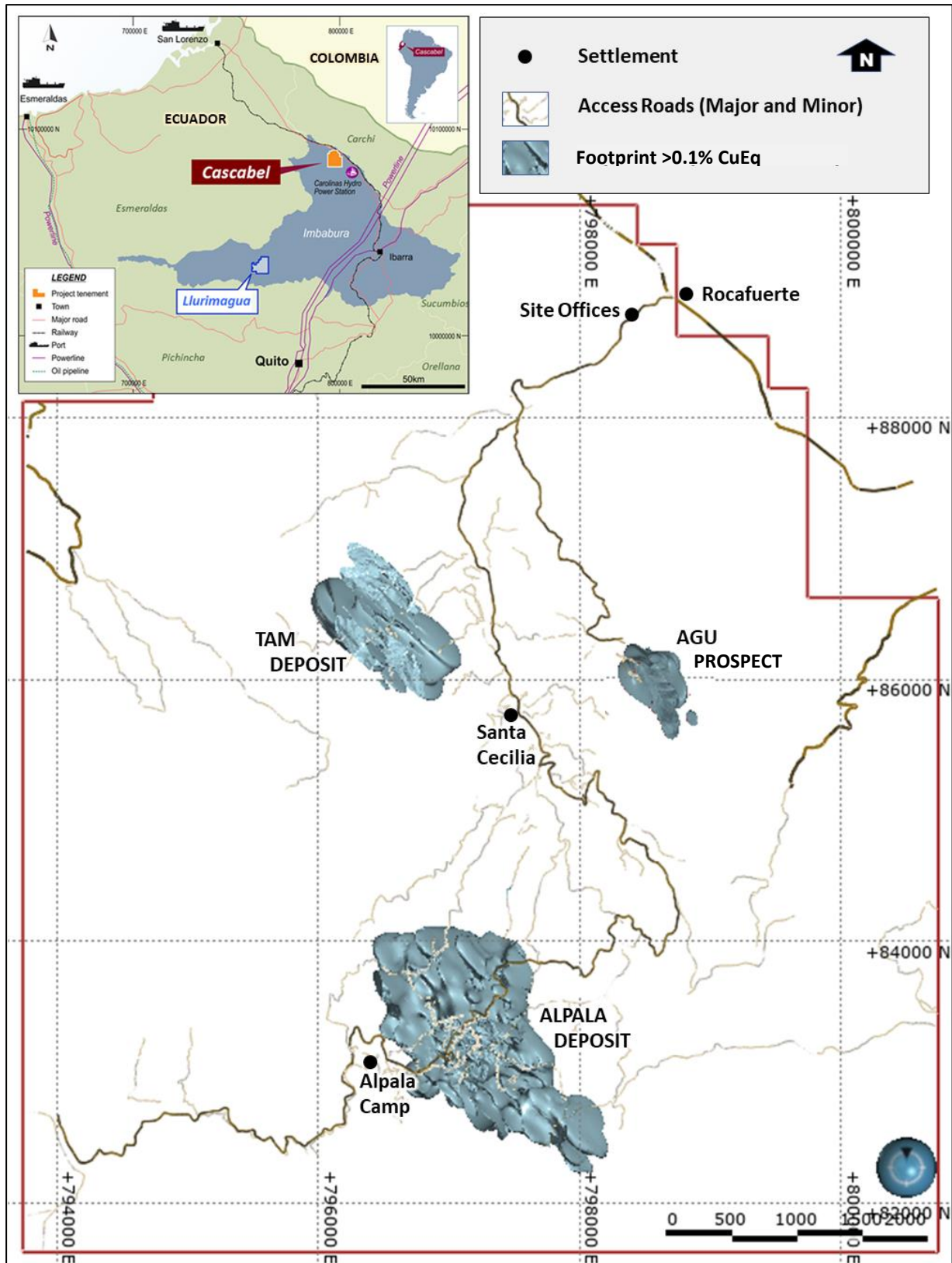
Figure 1: Location of TAM and Alpala deposits and Aguinaga target/prospect at the Cascabel project.
