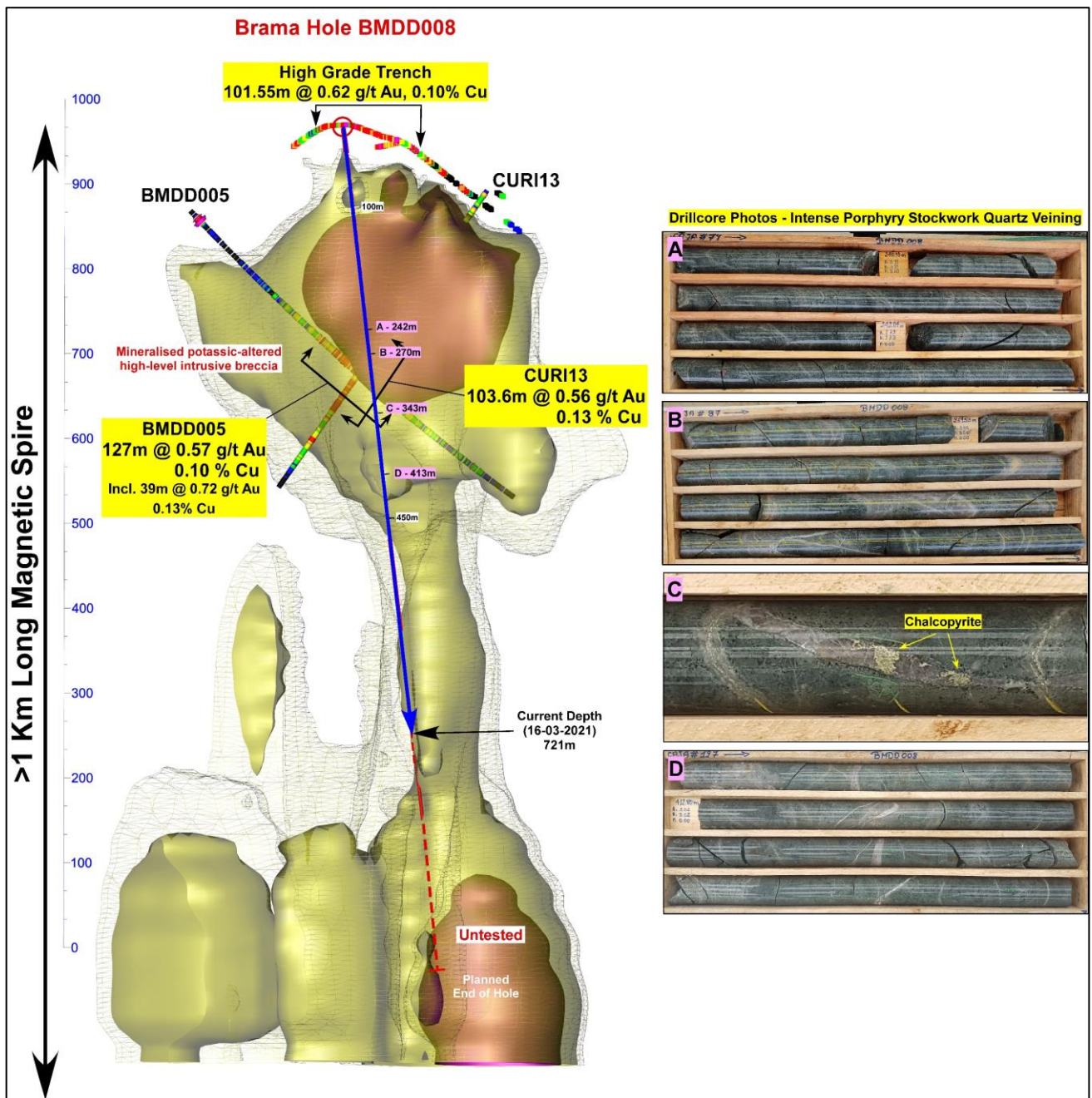
Figure 2: Brama 3-D magnetic model showing drill hole BMDD008, and progress to date. The interval from 100m – 450m is mineralized, and the drill hole is also targeting the broadening magnetic anomaly at a depth of >800m.
