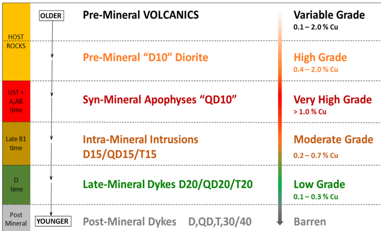
Figure 3: Geological units of the Alpala Deposit.
