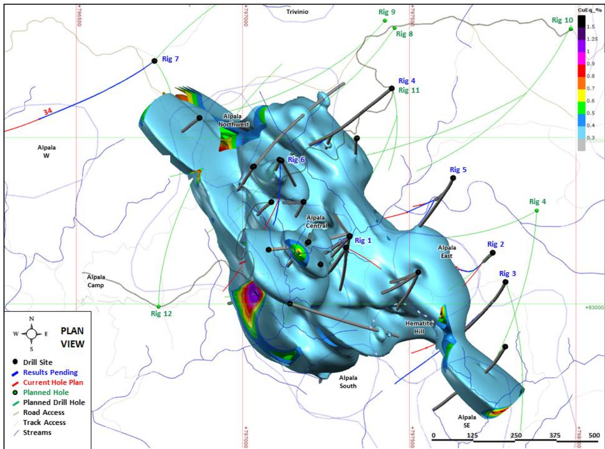
Figure 2: Plan view of the Alpala deposit showing CuEq cut-off grade shells from >0.3% CuEq to >1.5% CuEq. Drilling indicates a true width of the mineralized envelope at 0.3% CuEq cut-off grade, of up to 700 metres, a length in excess of 1300 metres and over 1800m vertical extent from surface.
