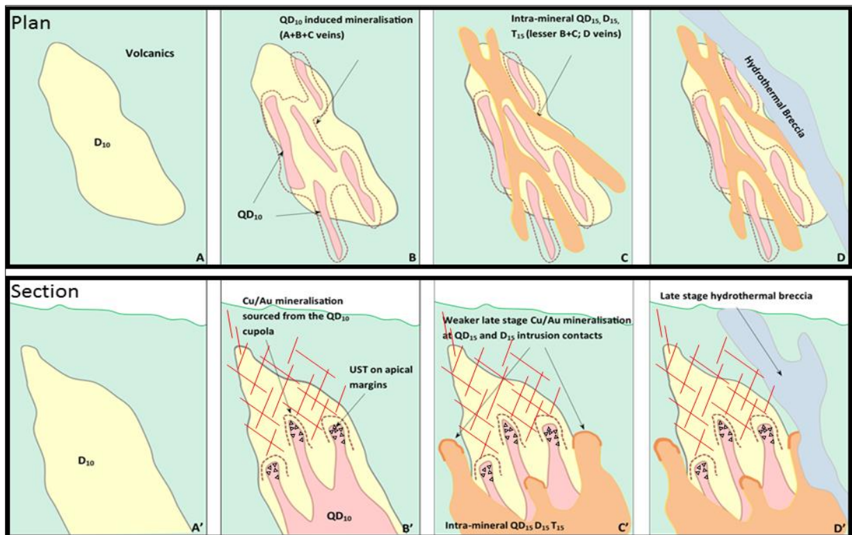
Figure 4: Alpala Genetic Model – schematic evolution of Alpala intrusive phases and associated vein paragenesis.
