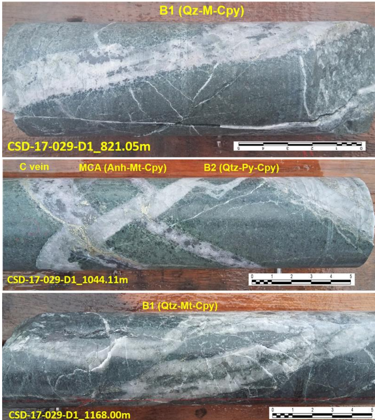
Figure 2: Selected examples of drill core intersected in Holes 29-D1, at Alpala Northwest.
