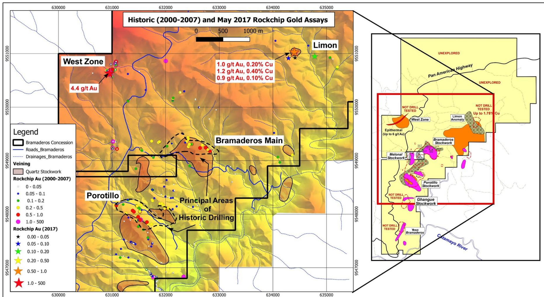
Figure showing the location of prospects and recent and historical rock chip sampling.
