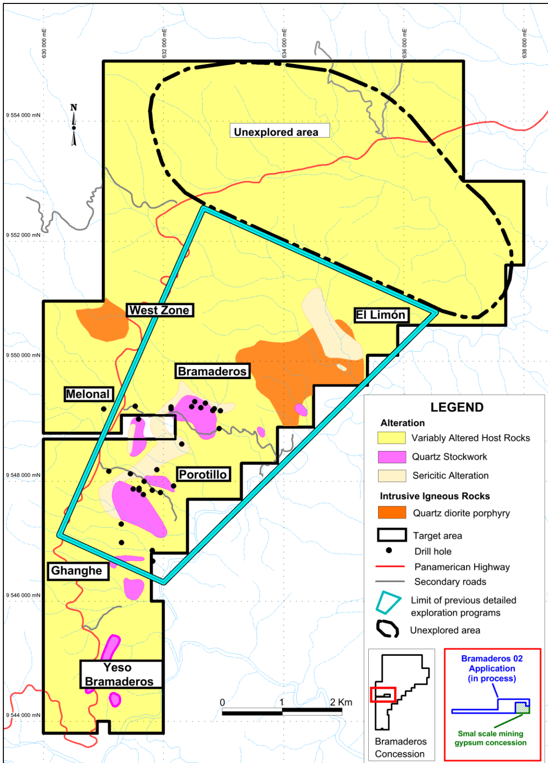
Figure 2. Bramaderos property. Geology, alteration, historical drill hole location and target areas
