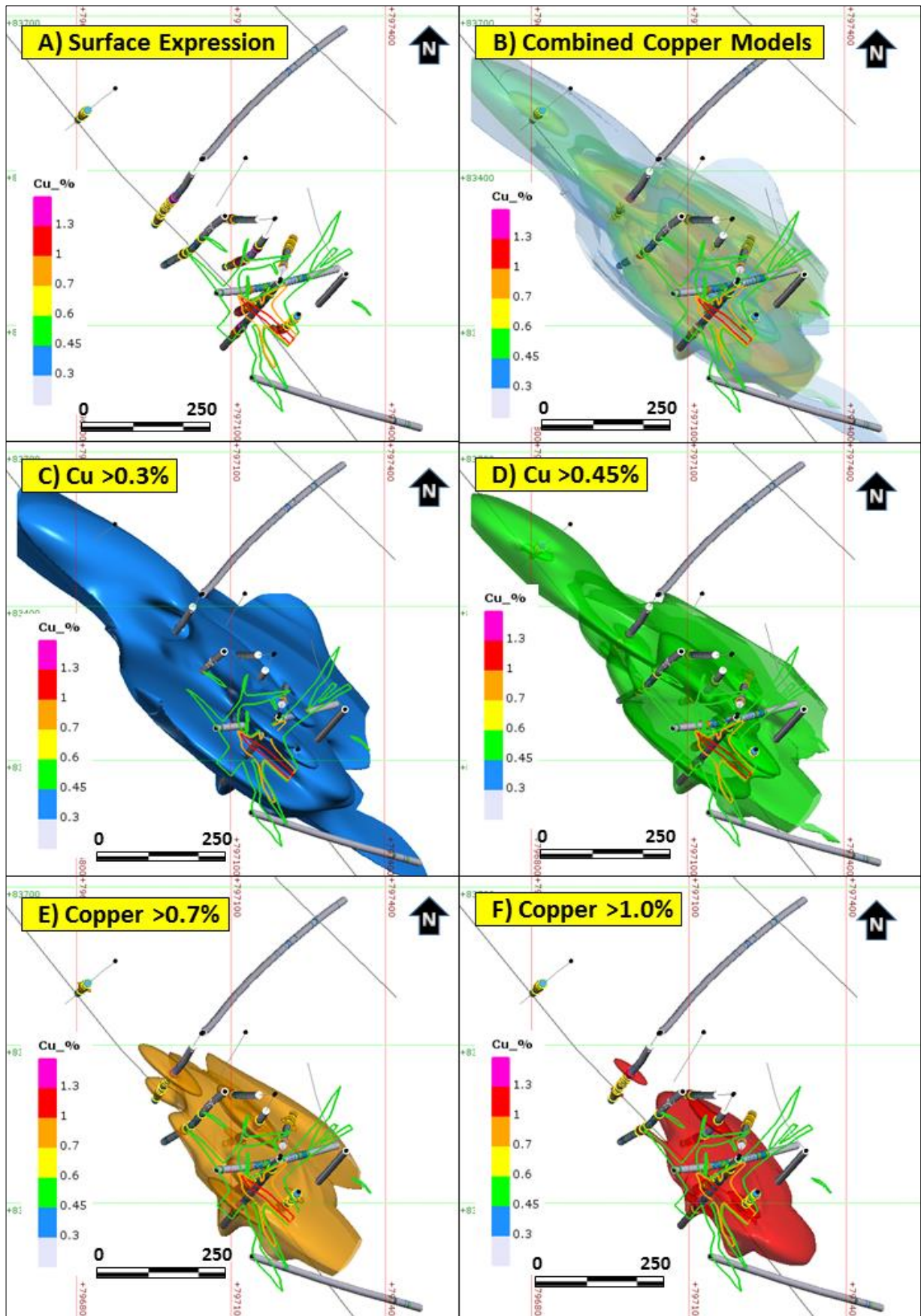
Figure 3: Preliminary copper modeling, showing abundance of B-type quartz veins on surface (A) and isosurfaces created at various copper cut-off grades (B to F).
