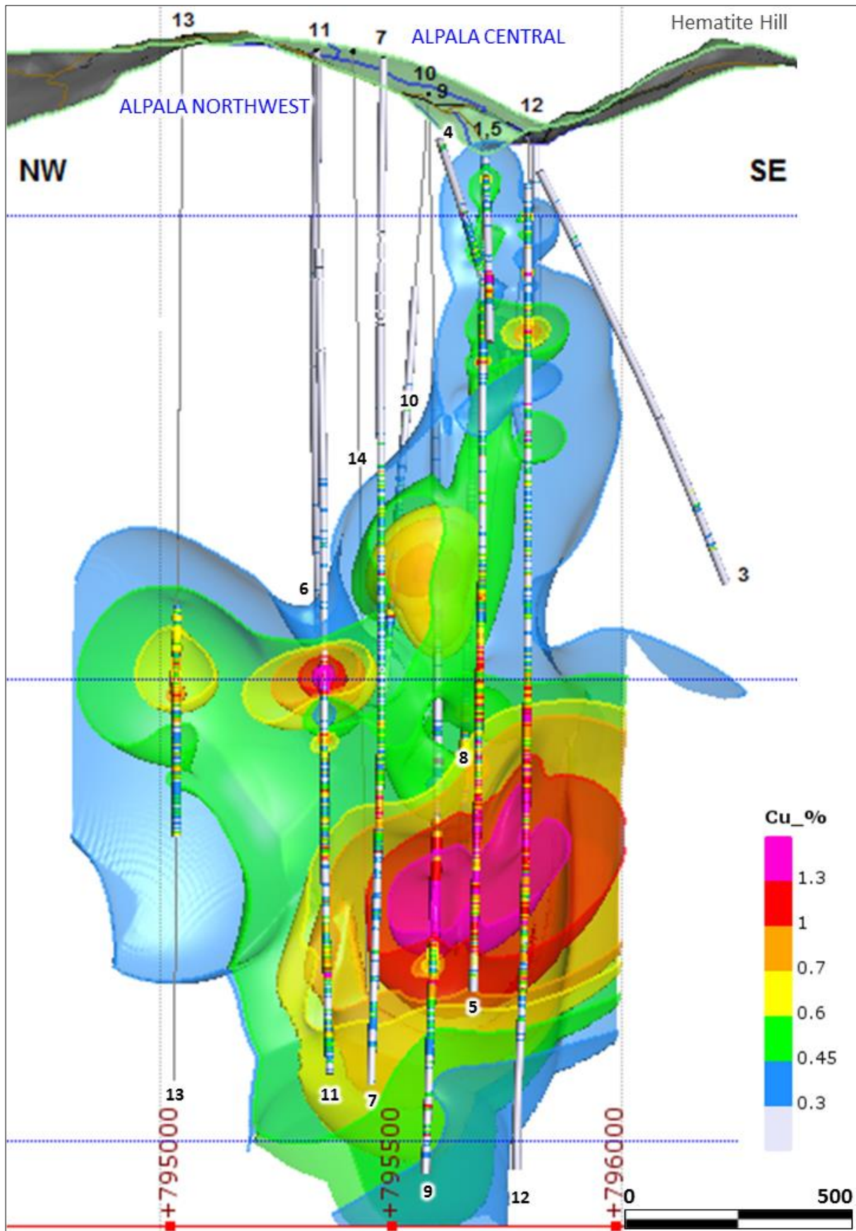
Figure 4: Northwest-southeast longitudinal section slice along the Alpa Structural Zone, showing the geometry of copper and gold mineralization defined by 3D copper modeling.
