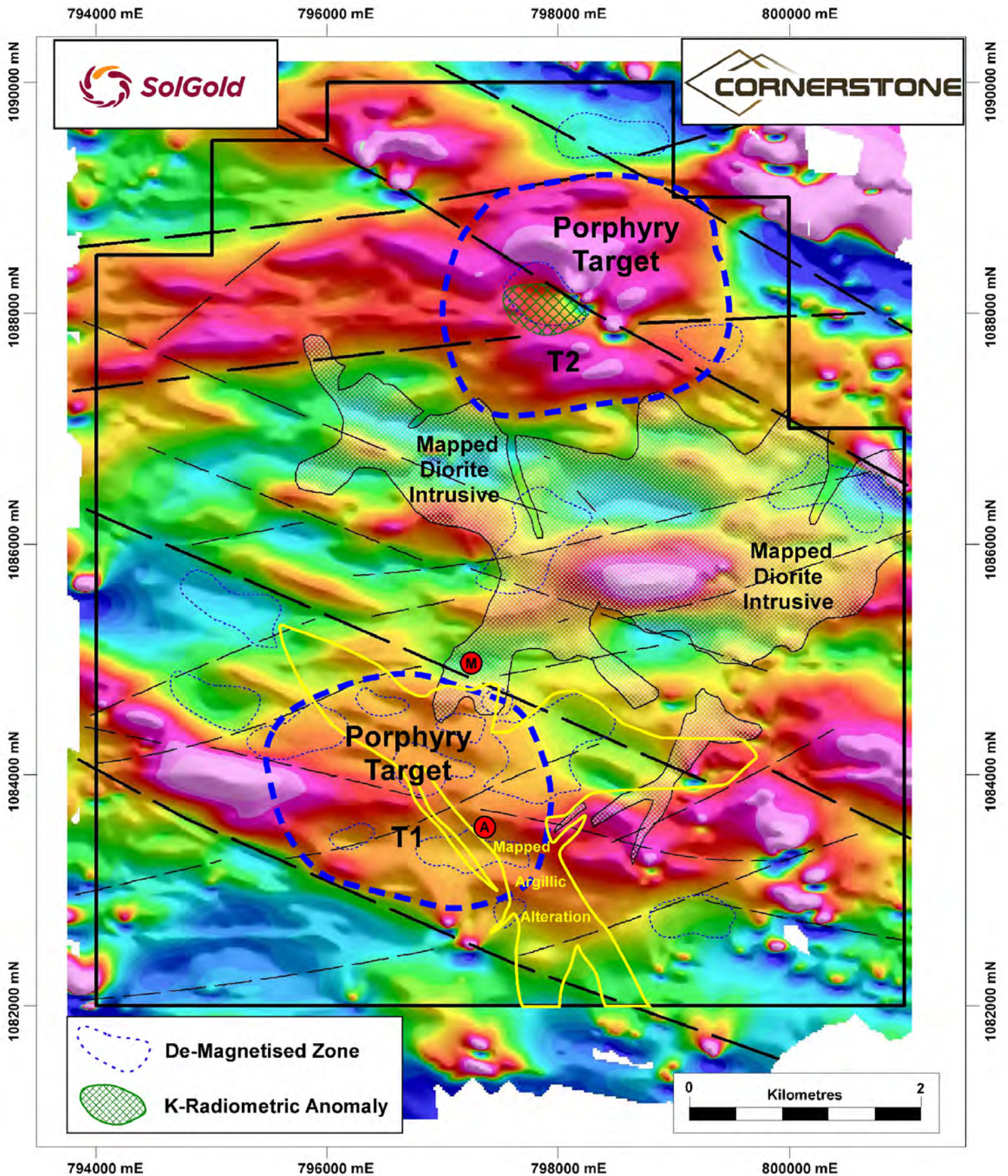
Figure 2: Magnetic imagery from the heli-magnetic survey (images are Reduced-to-Pole [RTP] images). The data are preliminary only and further processing is required to properly define domains of differing magnetic character. Preliminary interpretations define moderate magnetic intensity diorite domains (corresponding with mapped diorites), and weaker anomalies in areas of argillic ('clay') alteration. Strong northwest-trending structural domains are defined by alignment of anomalies.
